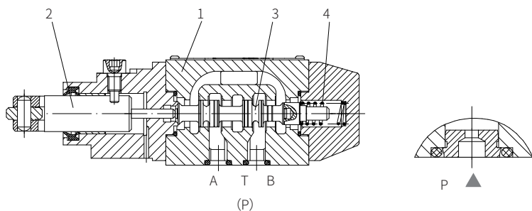
型号4WMR6E-5XJ/
